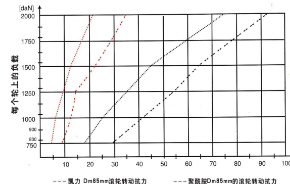
Rotation resistance of the roller of the Dm85mm Dm85mm
